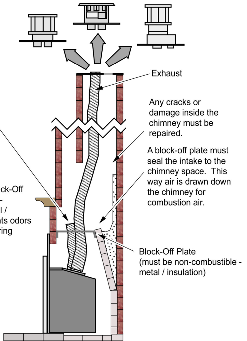
Masonry Fireplace
