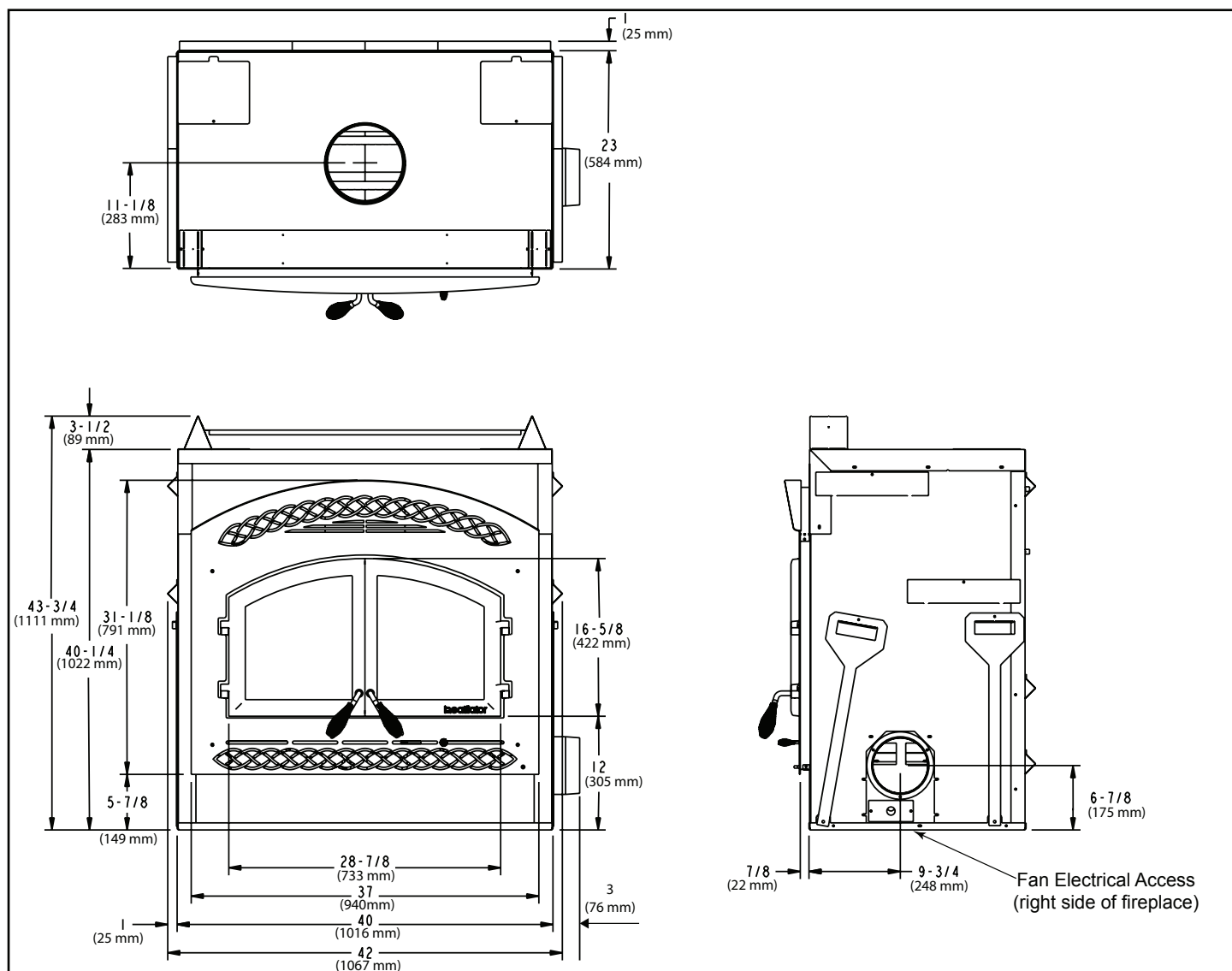
Figure 3.1 Fireplace Dimensions
