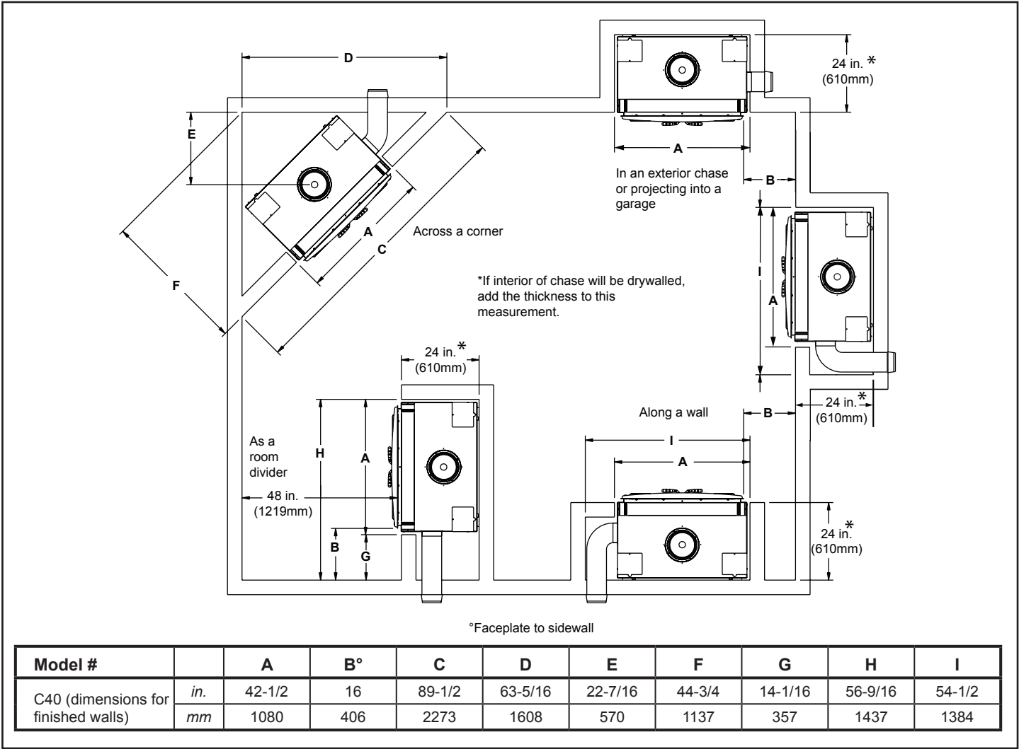
Figure 2.2 Fireplace Locations
