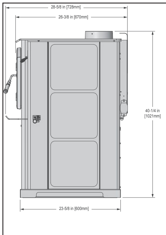
Figure 8.3 Side View
