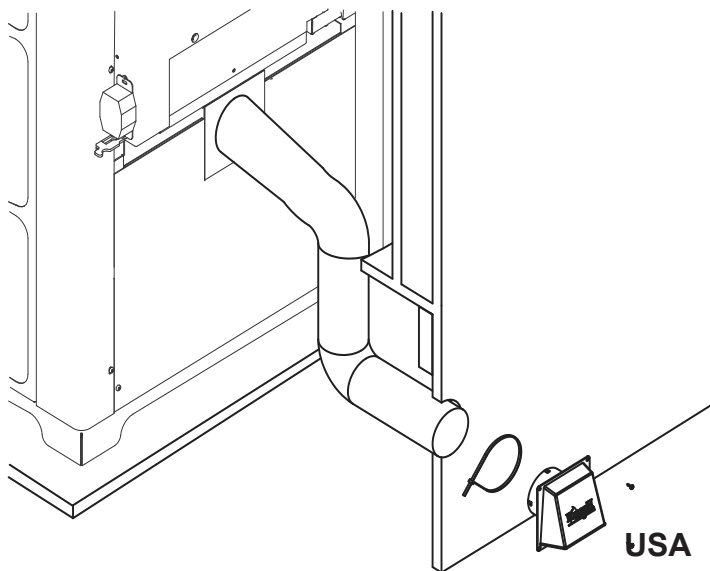
Figure 16.2 - Floor Installation
