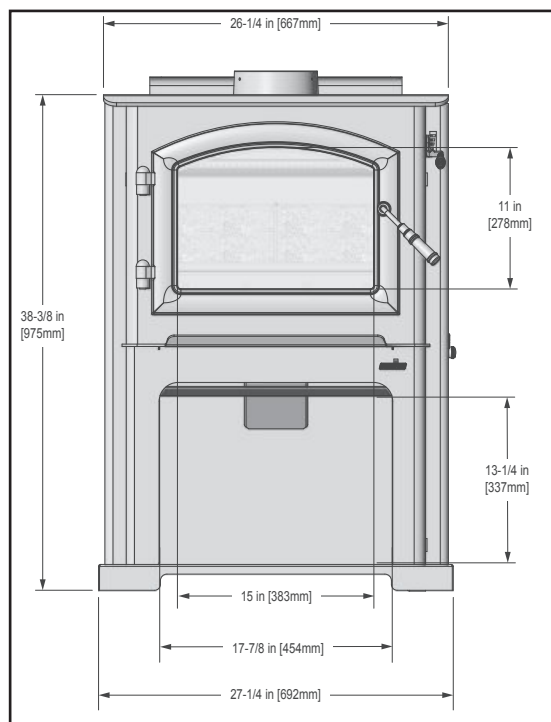
Figure 8.1 Front View
