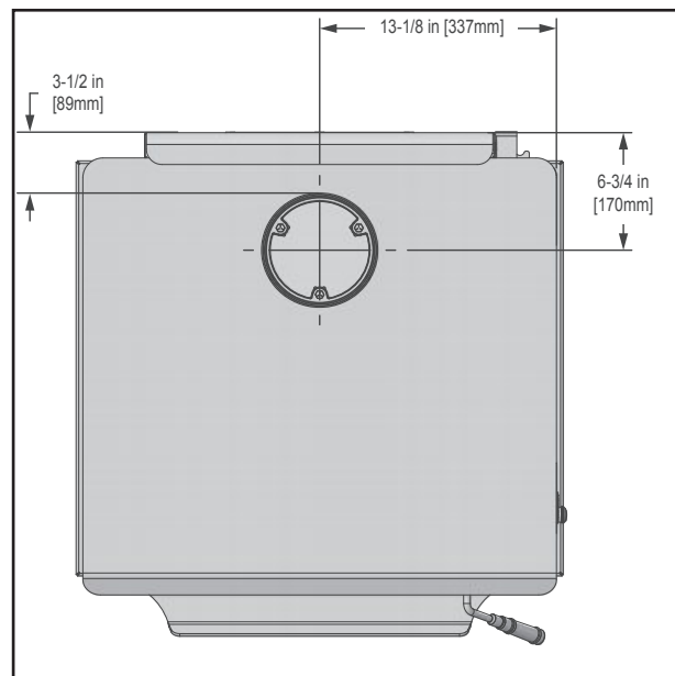
Figure 8.2 Top View
