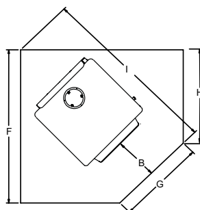
Corner Dimensions w/Double Wall Pipe
