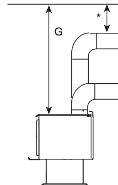
Stove to Ceiling Clearance
