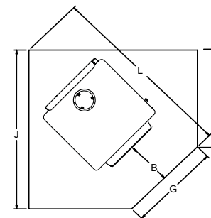
Corner Dimensions w/Single Wall Pipe
