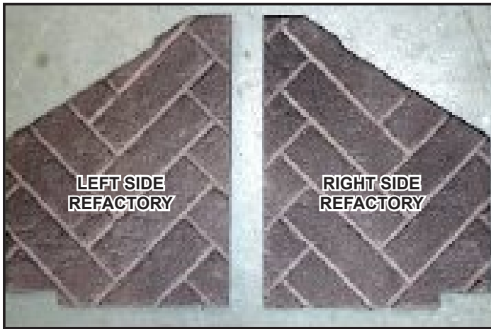
Figure 10.5 Refractory Components
