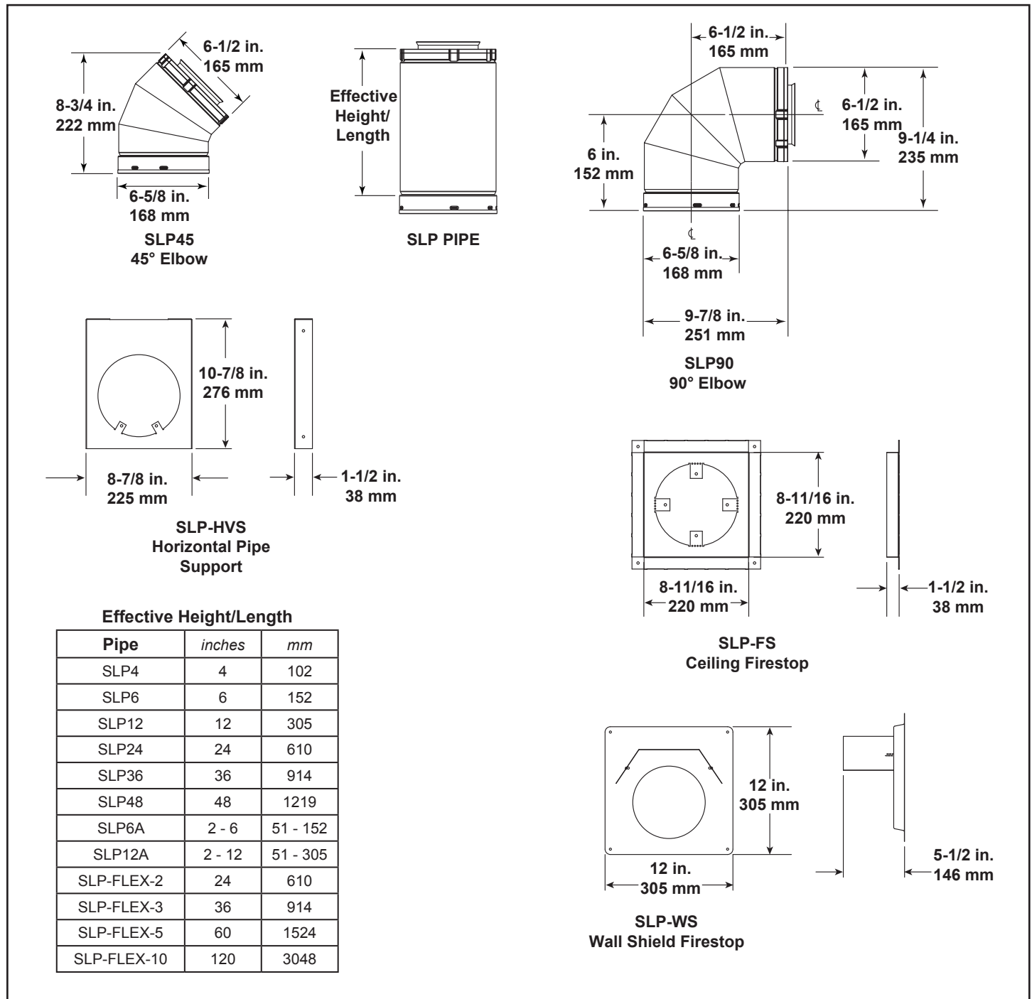
Figure 11.1 SLP Series Vent Components
