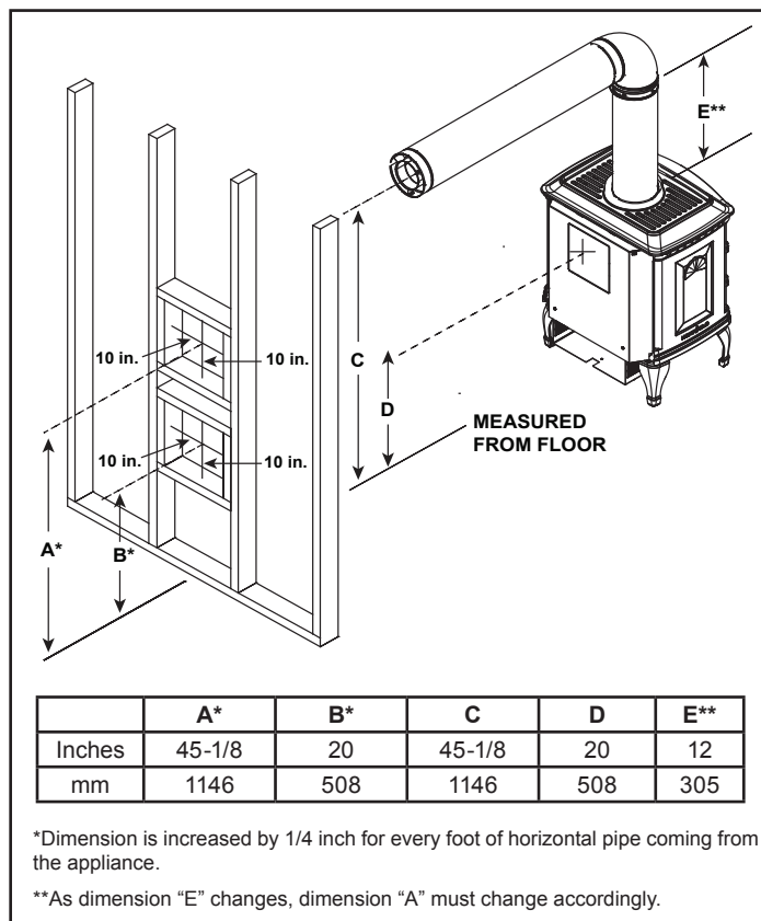
Figure 5.2 Wall Penetration
