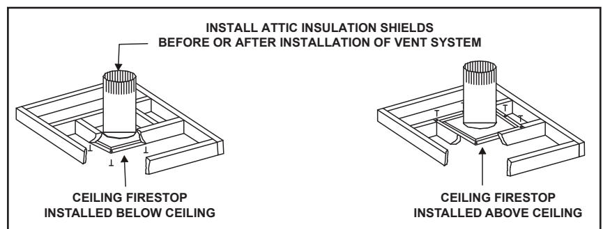
Figure 5.4 Installing the Attic Shield
