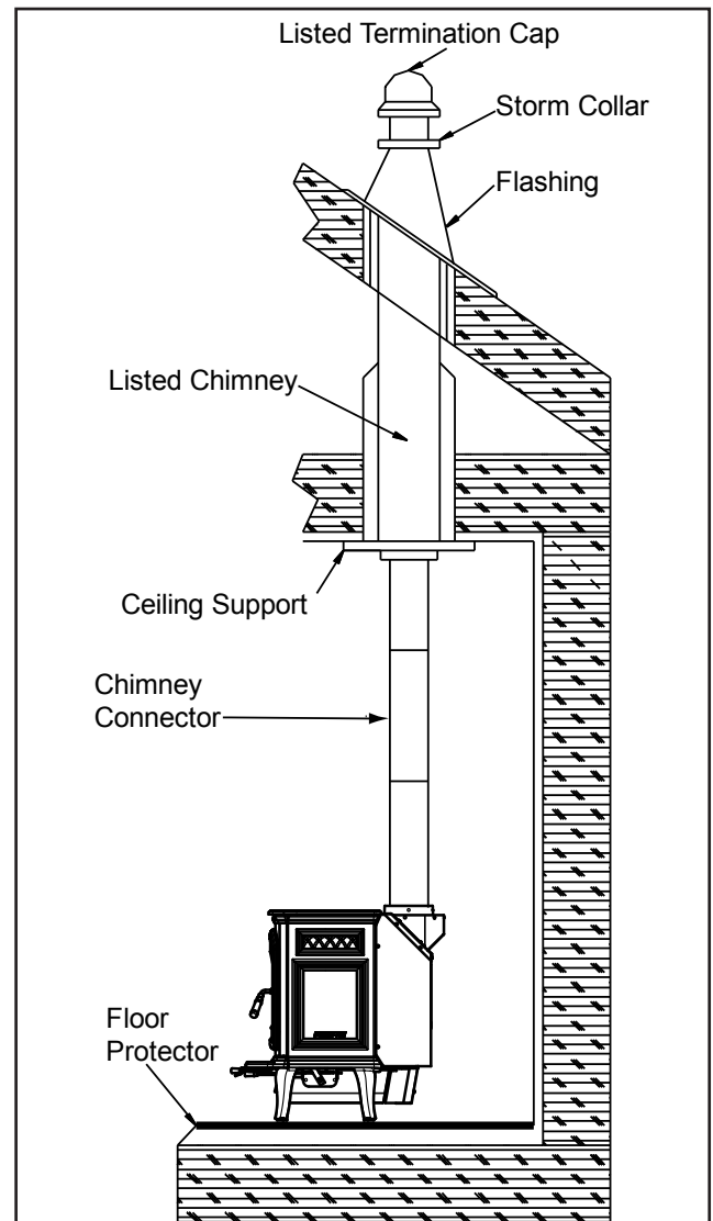
Figure 12.2 - Prefabricated Interior Chimney
