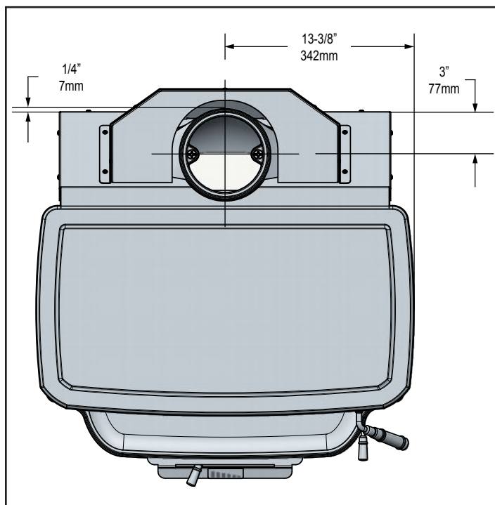
Figure 7.3 Top View
